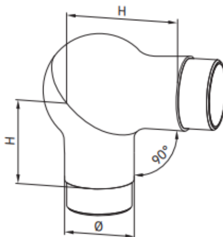
Codo conector para 2 tubos - (regulable)
