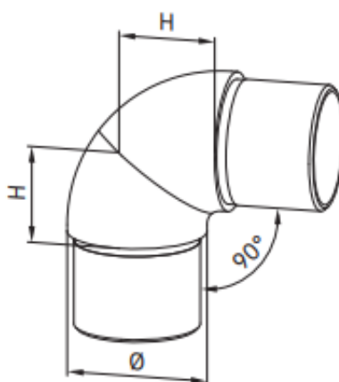
Codo conector para 2 tubos - (regulable)
